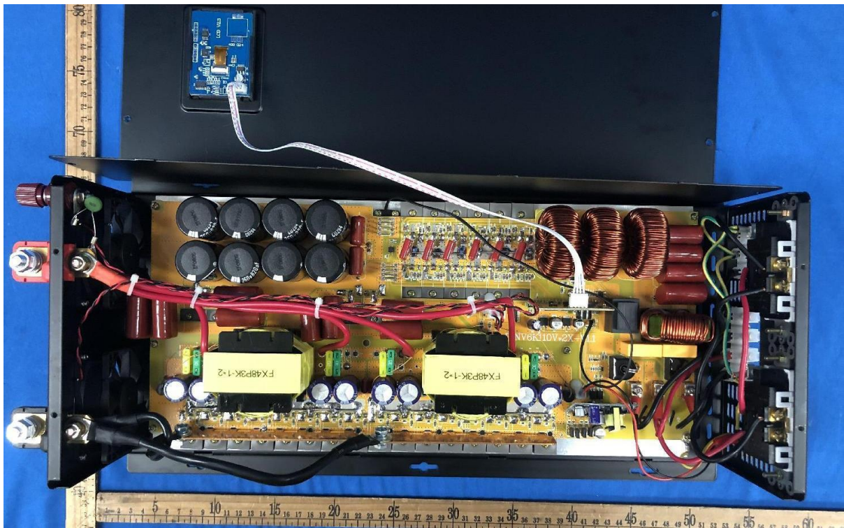
Fig 6. Internal view
